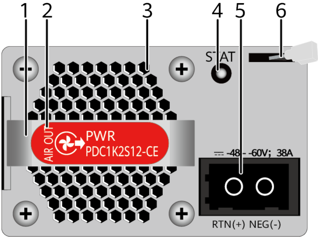
Figure 5-28 Panel of the PDC1K2S12-CE
