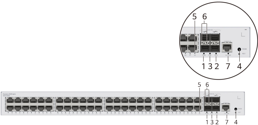
Figure 4-25 Indicators on the Switch
