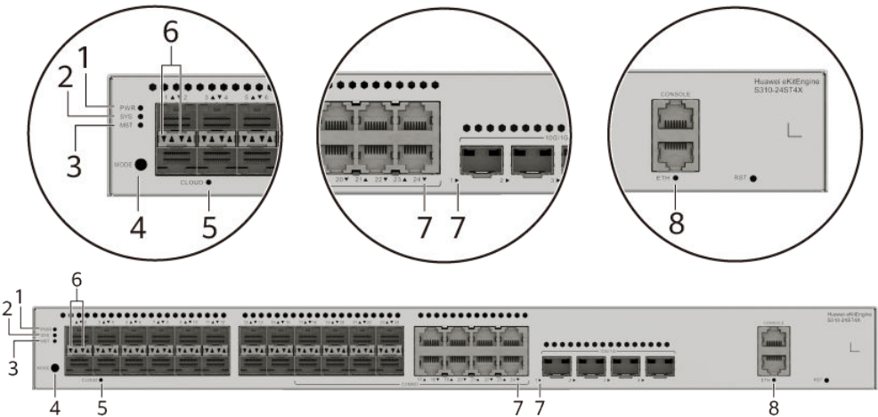
Figure 4-47 Indicators on the Switch
