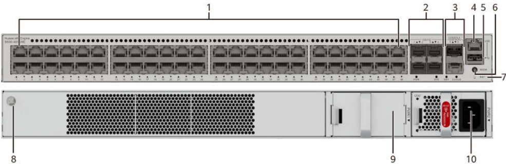
Figure 4-84 S530-48T4XE appearance
