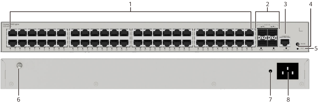
Figure 4-16 S220-48T4X appearance
