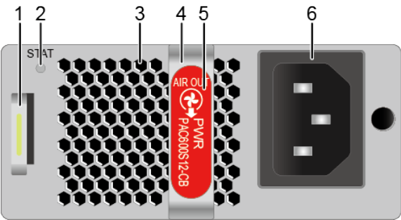
Figure 5-2 Panel of the PAC600S12-CB
