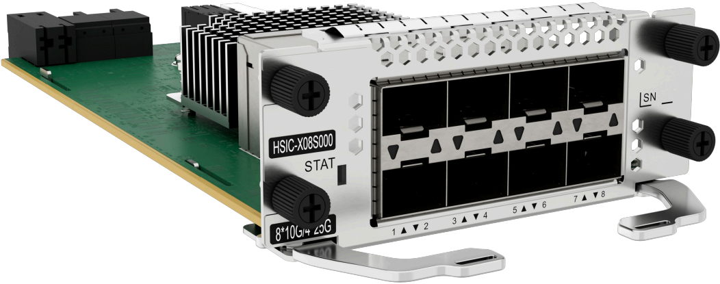
Figure 7-4 Appearance of the HSIC-X08S000
