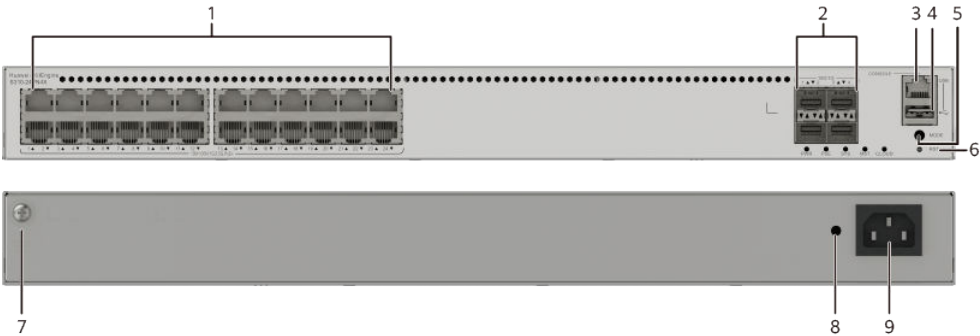
Figure 4-50 S310-24PN4X appearance
