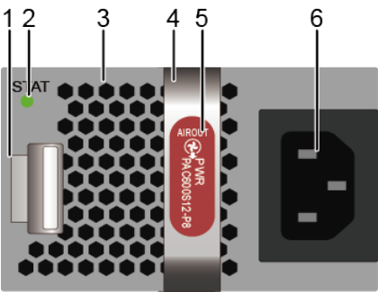
Figure 5-18 Panel of the PAC600S12-PB
