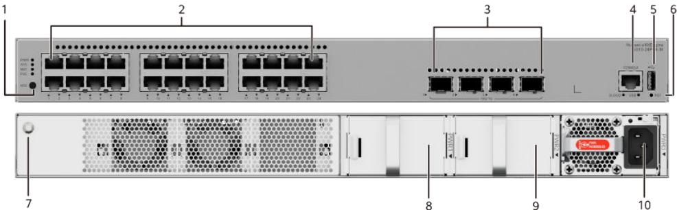
Figure 4-40 S310-24P4X-M appearance
