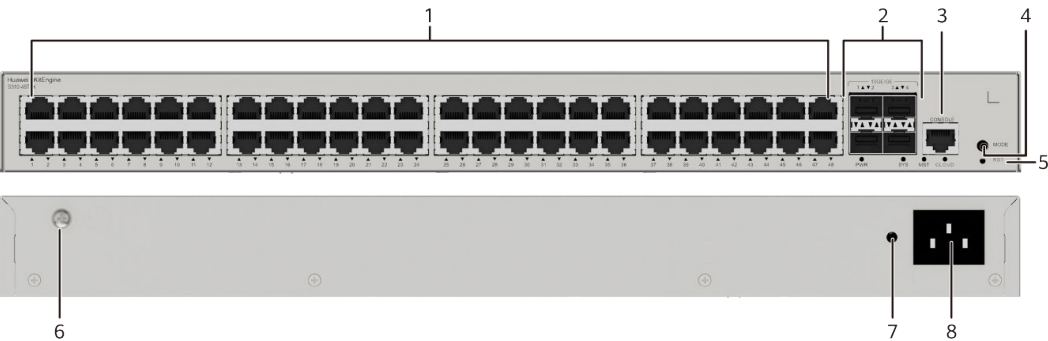
Figure 4-52 S310-48T4X appearance
