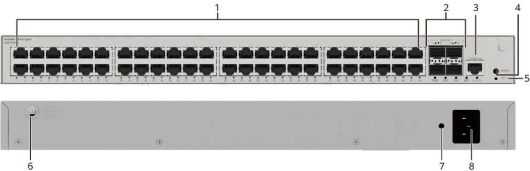
Figure 4-60 S310-48P4X appearance
