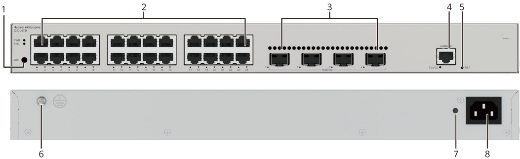
Figure 4-6 S220-24T4X appearance
