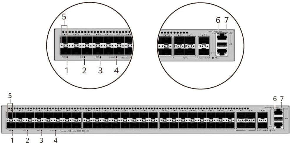
Figure 4-83 Indicators on the Switch
