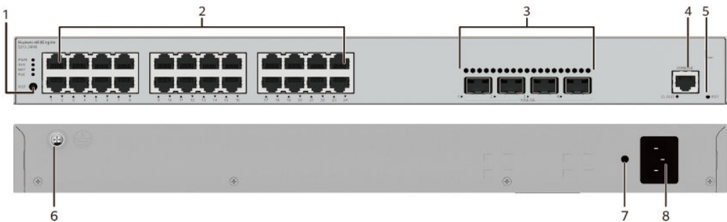
Figure 4-36 S310-24P4X appearance
