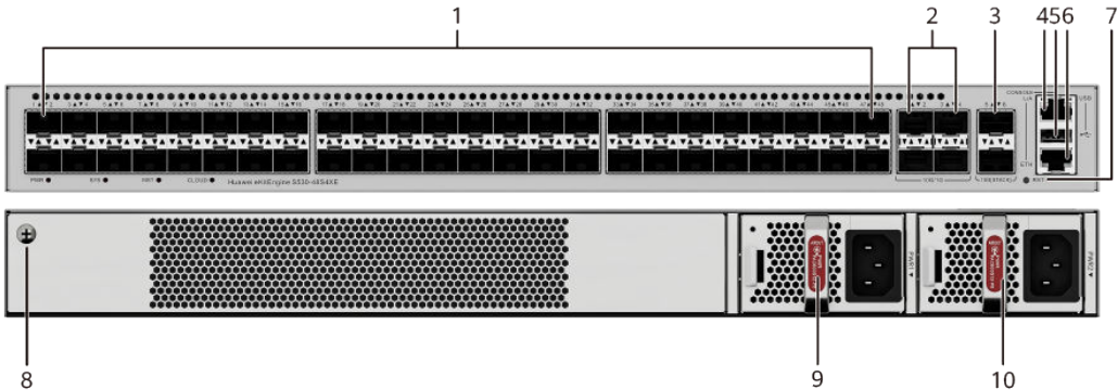
Figure 4-82 S530-48S4XE appearance
