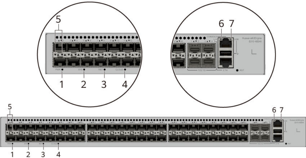
Figure 4-67 Indicators on the Switch
