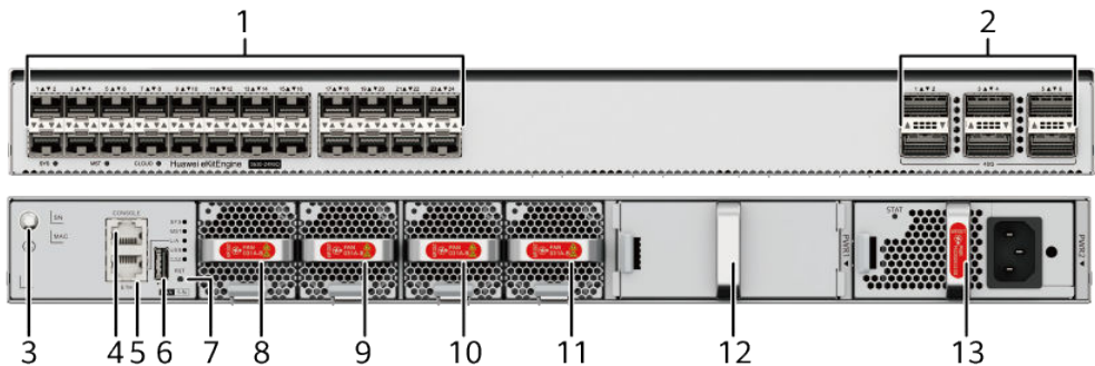
Figure 4-89 S630-24X6Q appearance
