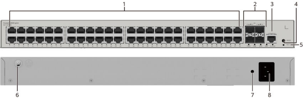
Figure 4-56 S310-48P4S appearance
