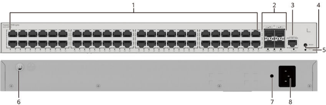
Figure 4-20 S220-48P4S appearance
