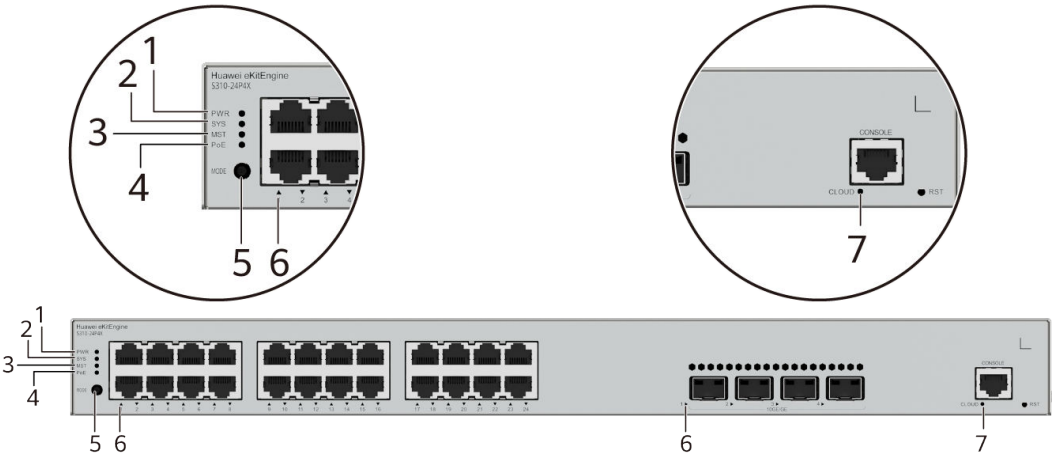
Figure 4-37 Indicators on the Switch
