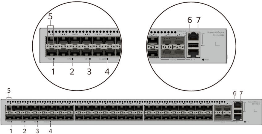
Figure 4-69 Indicators on the Switch
