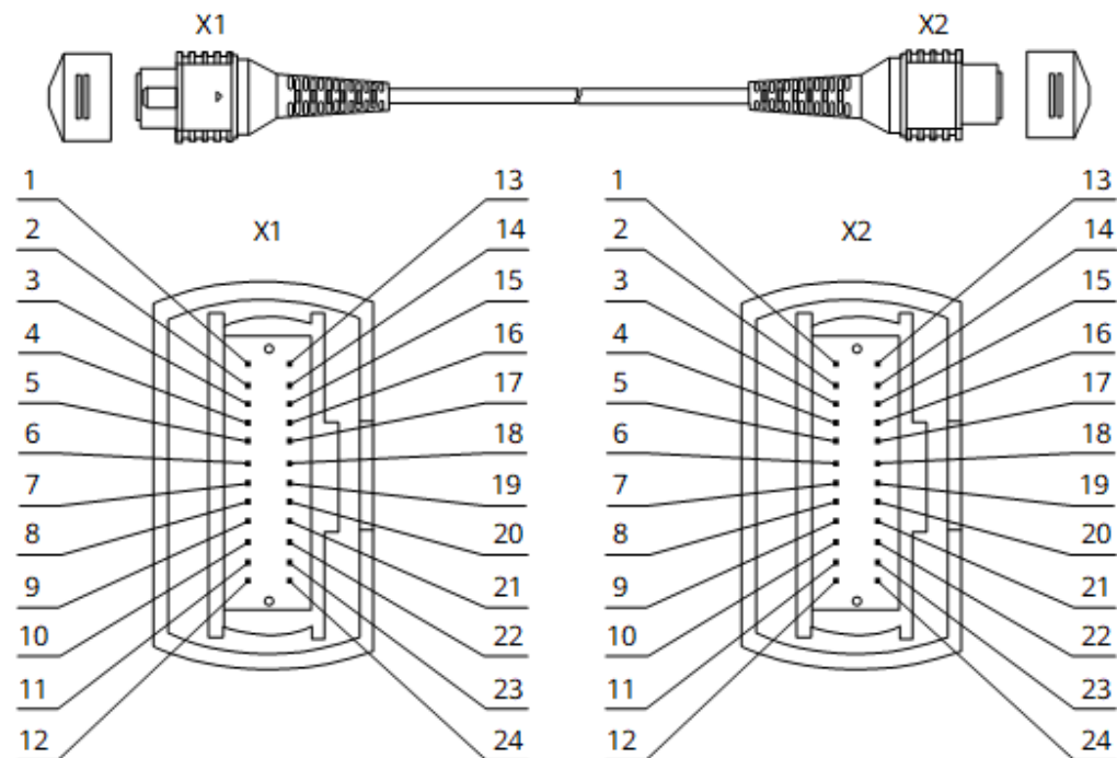
Figure 8-13 Structure of a 24-strand MPO-MPO fiber jumper
