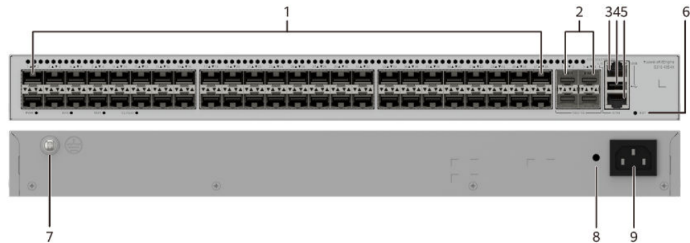
Figure 4-66 S310-48S4X appearance
