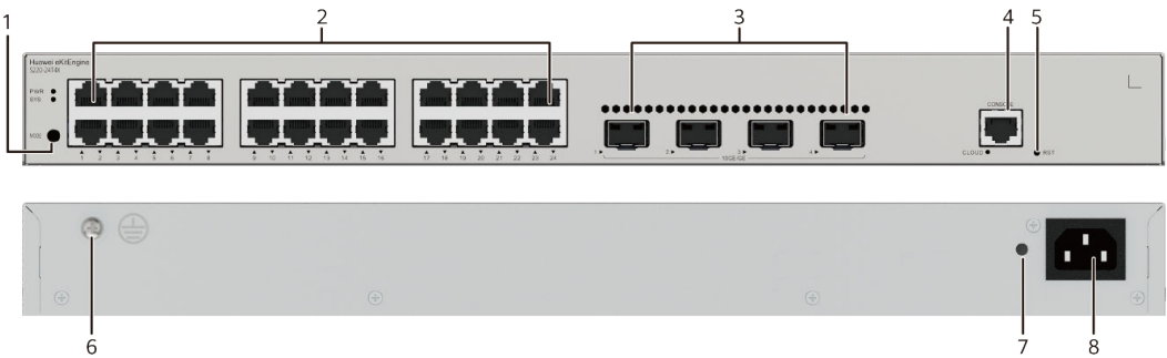
Figure 4-8 S220-24T4X appearance
