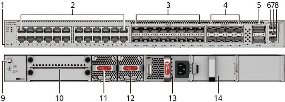
Figure 4-87 S620-24T16X8Y2CZ appearance
