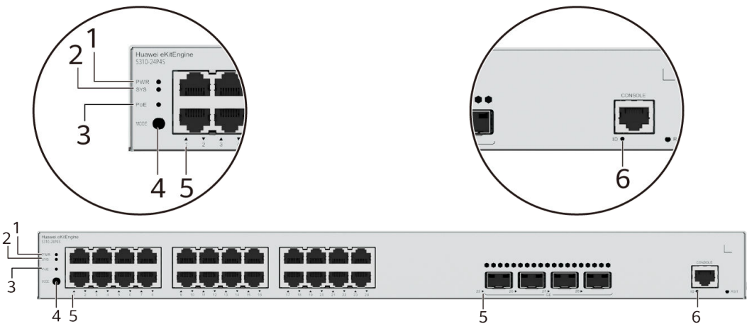
Figure 4-31 Indicators on the Switch
