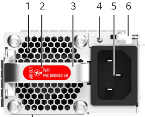
Figure 5-22 Panel of the PAC1000S56-EB
