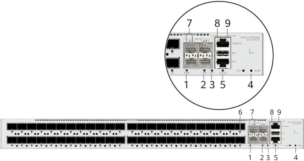
Figure 4-49 Indicators on the Switch
