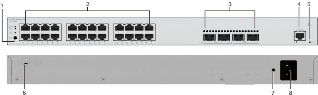
Figure 4-28 S310-24P4S appearance
