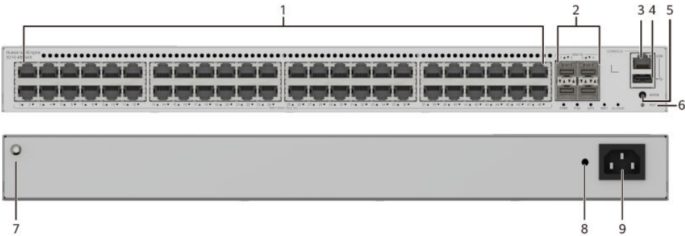
Figure 4-74 S310-48PN4X appearance
