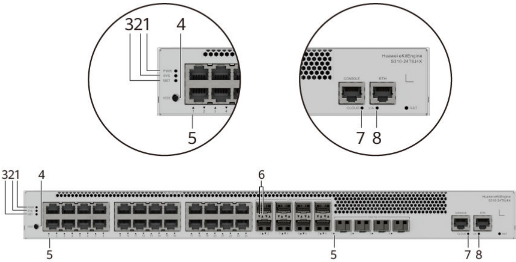
Figure 4-65 Indicators on the Switch
