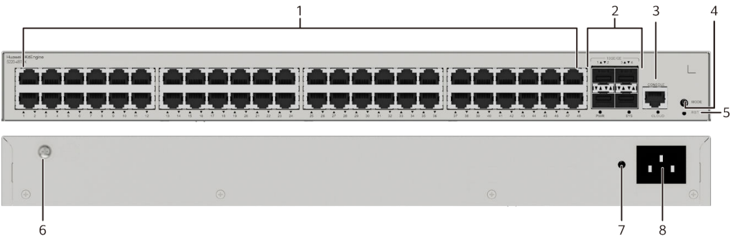
Figure 4-18 S220-48T4X appearance
