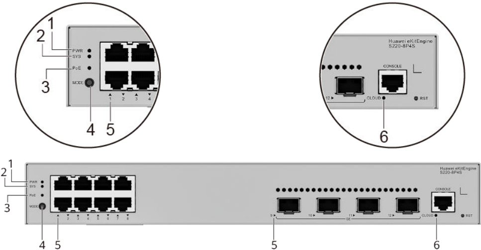
Figure 4-3 Indicators on the Switch
