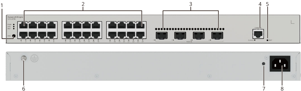
Figure 4-32 S310-24T4X appearance
