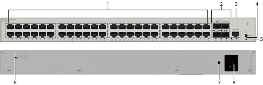
Figure 4-58 S310-48P4X appearance
