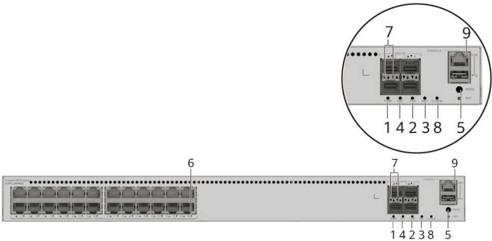
Figure 4-51 Indicators on the Switch
