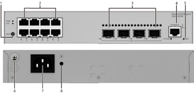
Figure 4-2 S220-8T4S appearance
