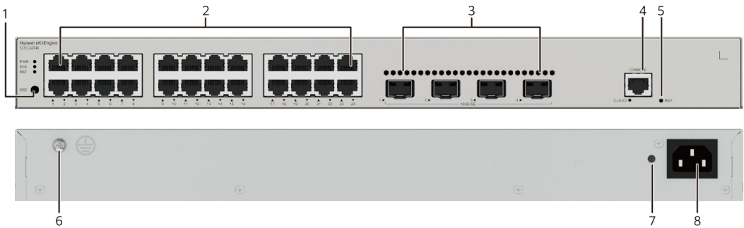
Figure 4-34 S310-24T4X appearance
