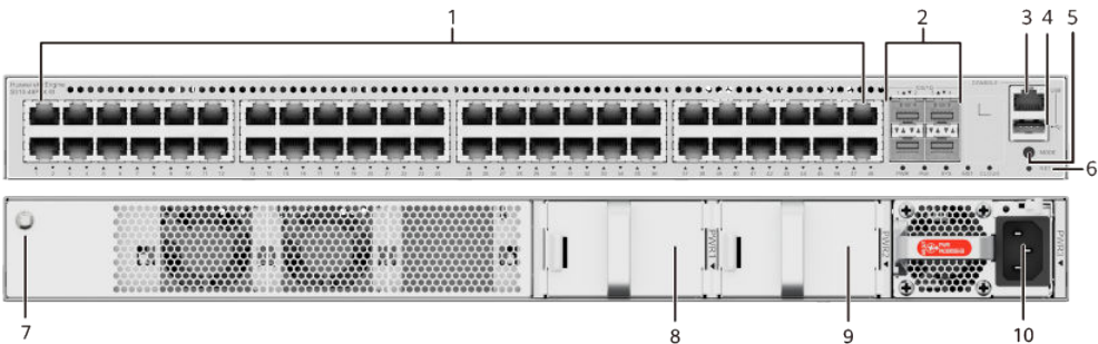
Figure 4-62 S310-48P4X-M appearance
