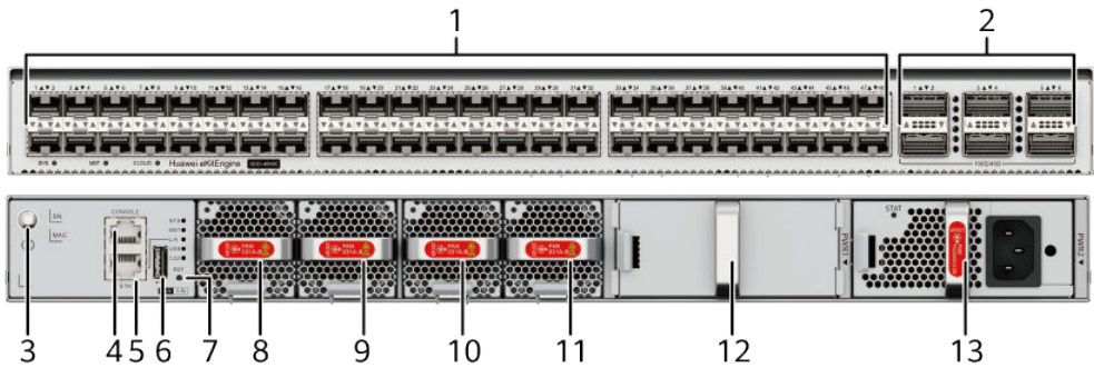
Figure 4-95 S630-48X6C appearance
