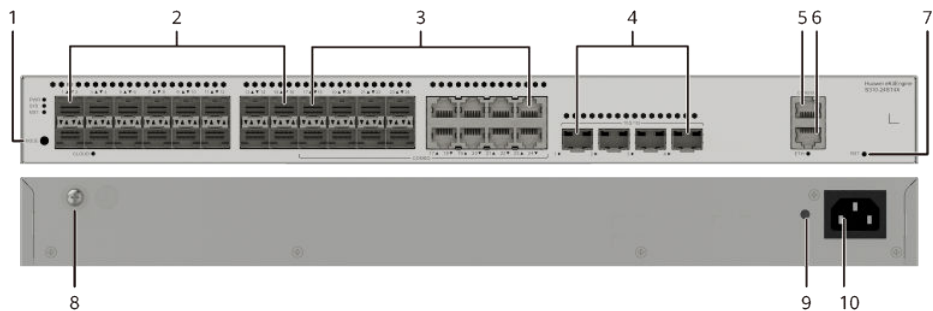
Figure 4-44 S310-24ST4X appearance
