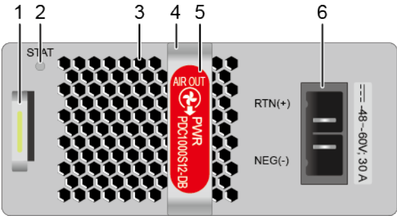
Figure 5-8 Panel of the PDC1000S12-DB
