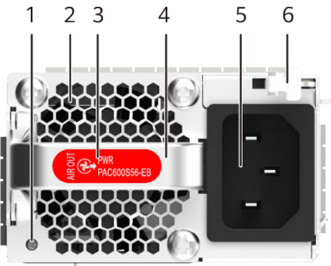
Figure 5-20 Panel of the PAC600S56-EB
