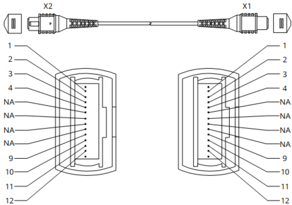
Figure 8-11 Structure of an 8-strand MPO-MPO fiber jumper
