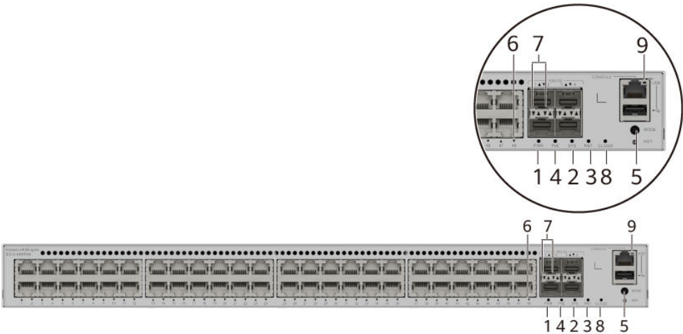
Figure 4-73 Indicators on the Switch
