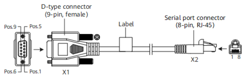
Figure 8-25 Structure of a console cable
