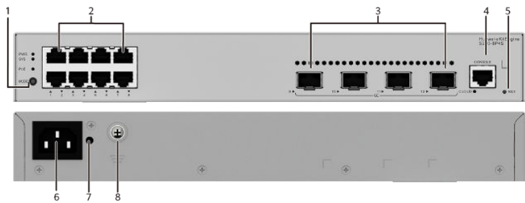
Figure 4-4 S220-8P4S appearance
