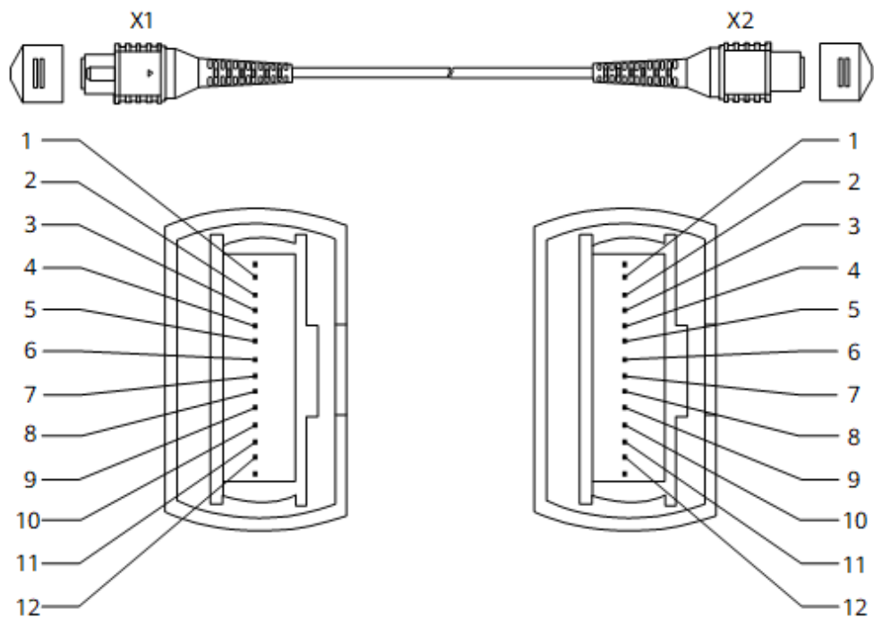
Figure 8-12 Structure of a 12-strand MPO-MPO fiber jumper
