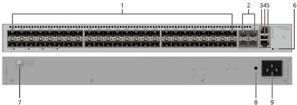
Figure 4-68 S310-48S4X appearance
