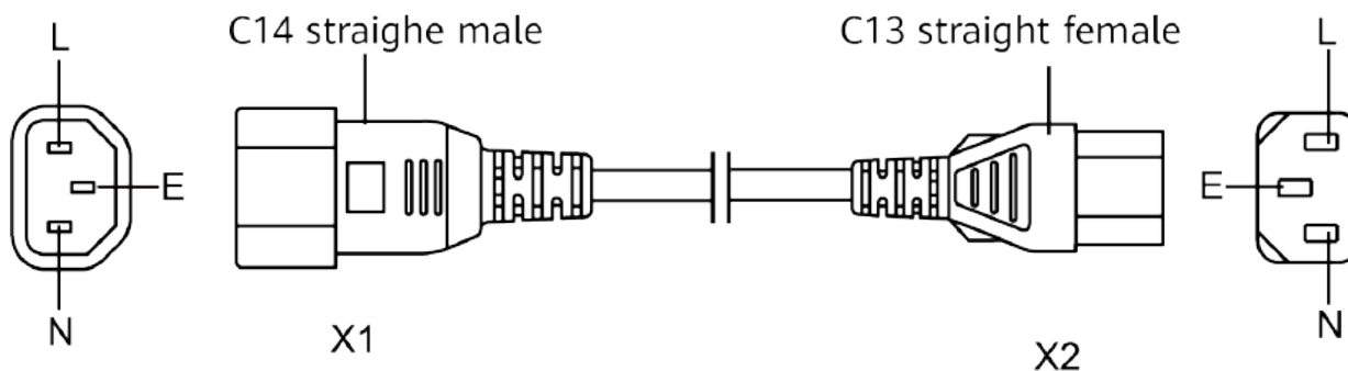
Figure 8-21 Structure of a C14 straight male to C13 straight female AC power cable
