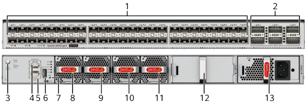
Figure 4-93 S630-48X6Q appearance
