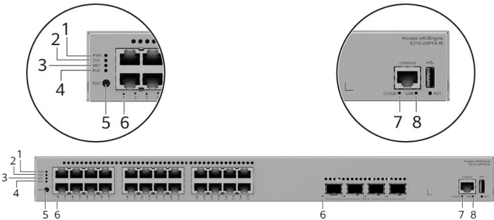
Figure 4-41 Indicators on the Switch
