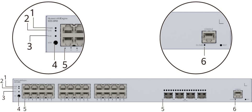
Figure 4-7 Indicators on the Switch
