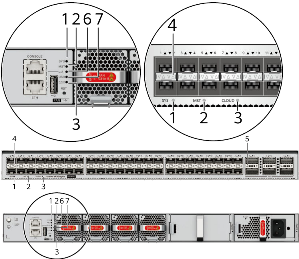
Figure 4-90 Indicators on the switch
