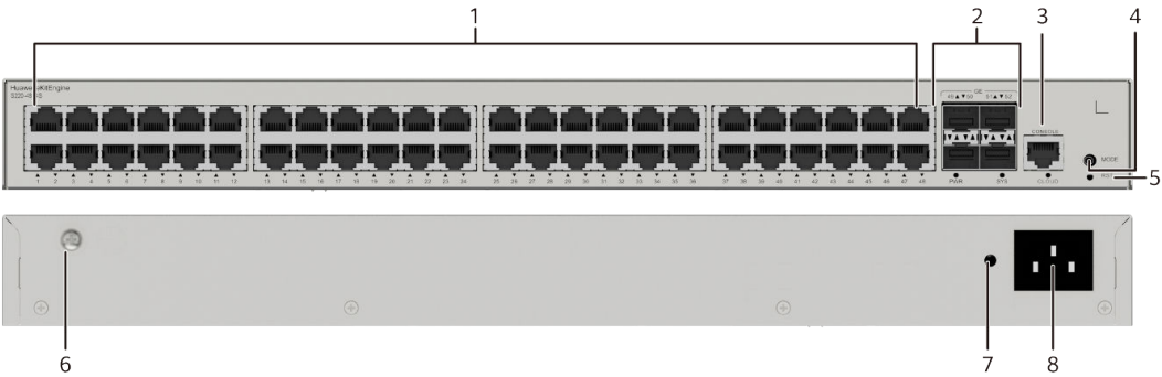
Figure 4-14 S220-48T4S appearance
