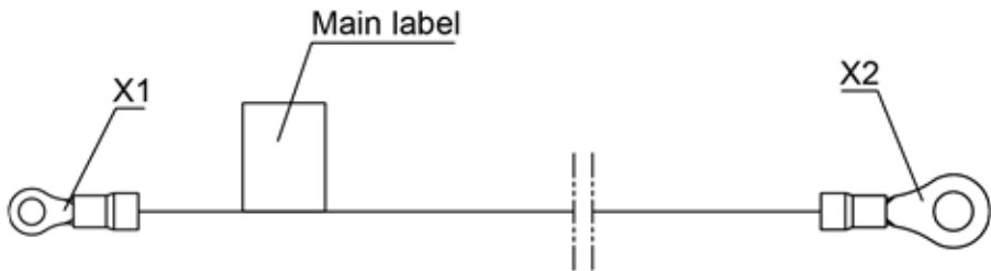
Figure 8-2 Structure of a ground cable
