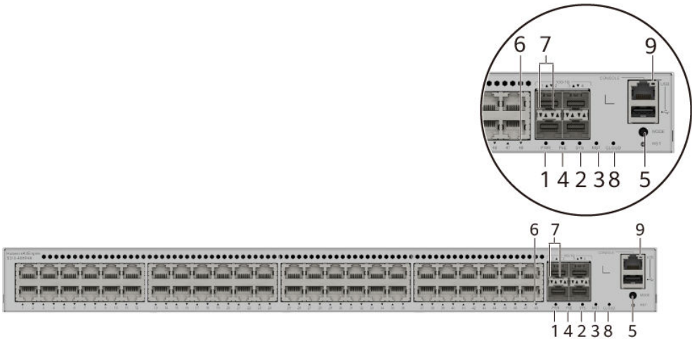
Figure 4-75 Indicators on the Switch
