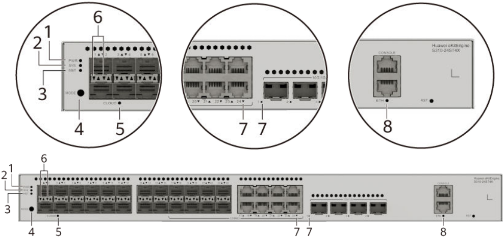
Figure 4-45 Indicators on the Switch
