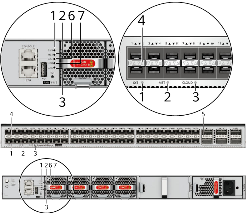
Figure 4-94 Indicators on the switch
