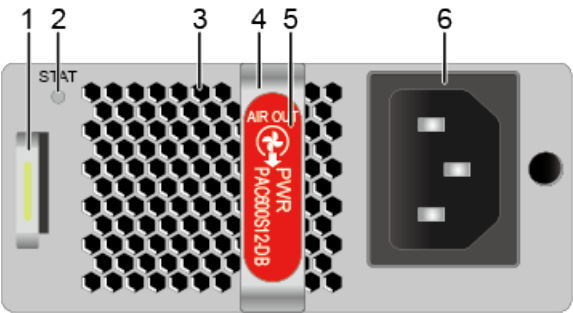
Figure 5-4 Panel of the PAC600S12-DB
