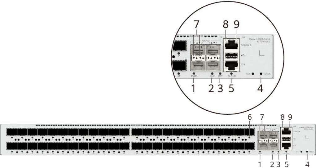
Figure 4-71 Indicators on the Switch
