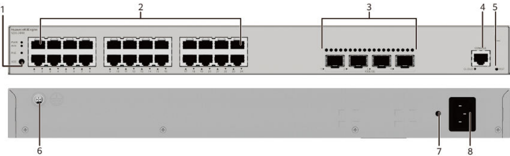
Figure 4-10 S220-24P4X appearance
