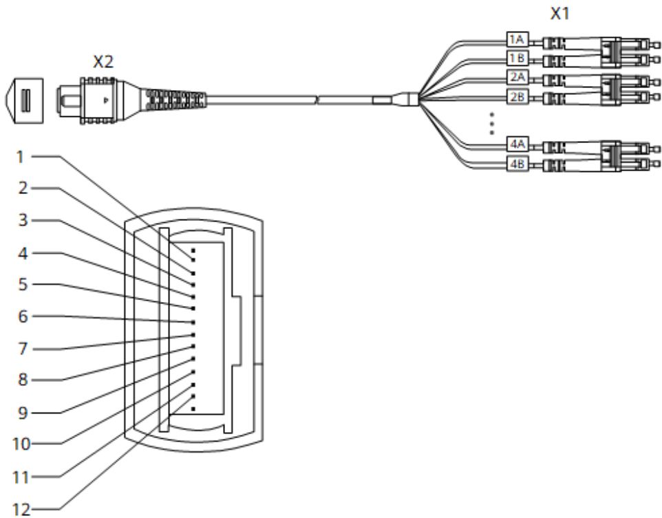
Figure 8-14 Structure of an MPO-4*DLC fiber jumper
