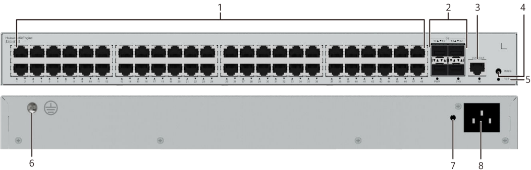
Figure 4-30 S310-48T4S appearance
