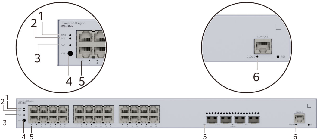
Figure 4-13 Indicators on the Switch
