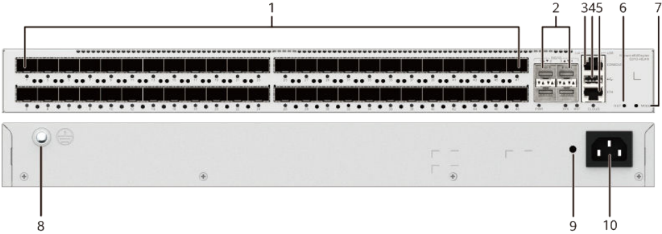
Figure 4-70 S310-48J4X appearance
