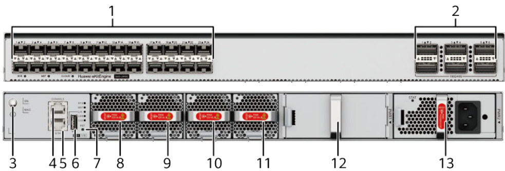
Figure 4-91 S630-24X6C appearance
