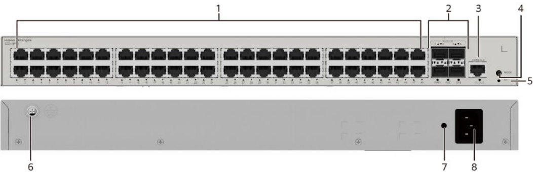
Figure 4-24 S220-48P4X appearance
