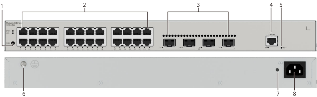
Figure 4-26 S310-24T4S appearance
