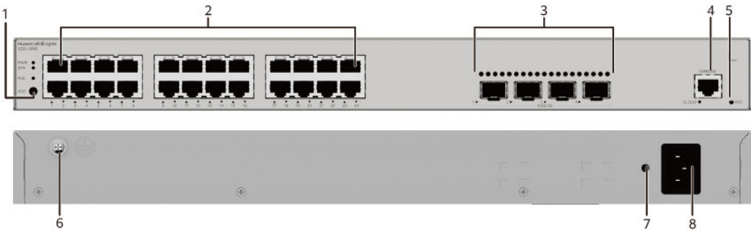
Figure 4-12 S220-24P4X appearance
