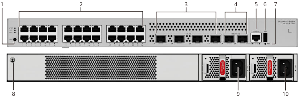
Figure 4-76 S530-24T4XE appearance
