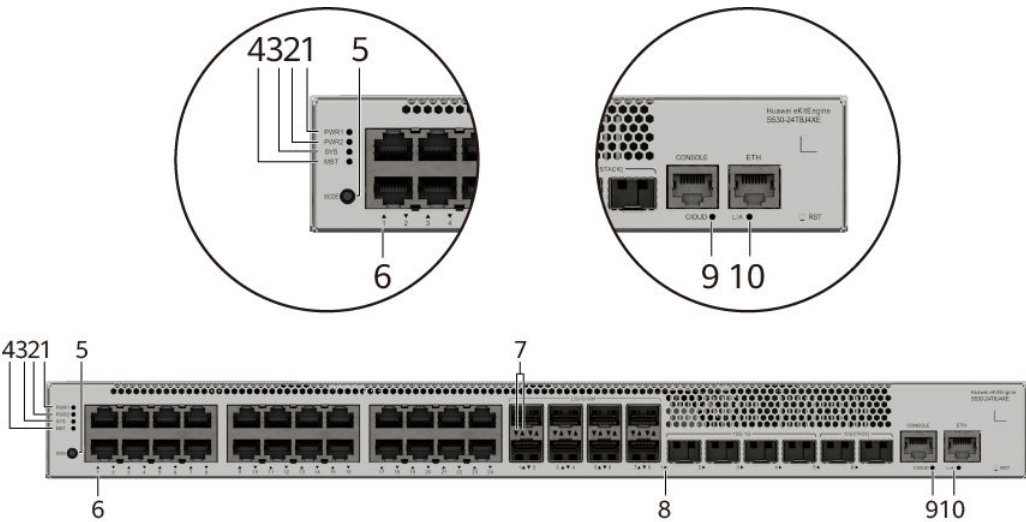
Figure 4-79 Indicators on the Switch
