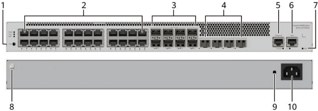
Figure 4-64 S310-24T8J4X appearance
