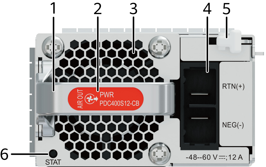
Figure 5-16 Panel of the PDC400S12-CB
