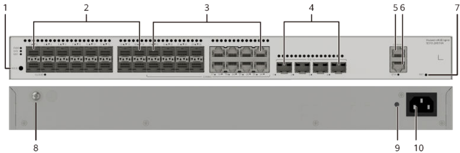
Figure 4-46 S310-24ST4X appearance
