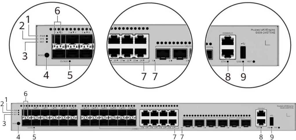
Figure 4-81 Indicators on the Switch
