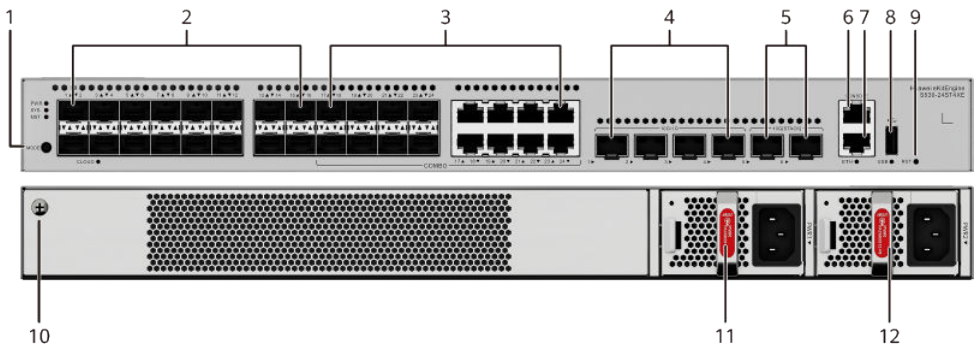
Figure 4-80 S530-24ST4XE appearance
