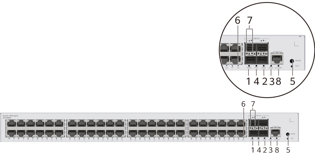
Figure 4-55 Indicators on the Switch
