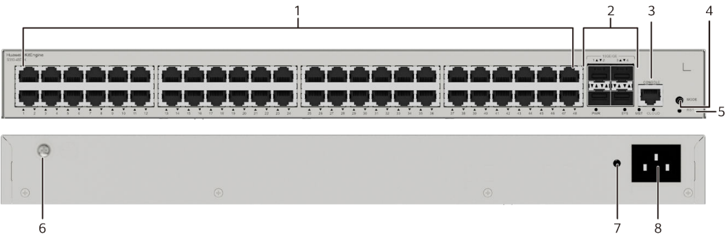
Figure 4-54 S310-48T4X appearance
