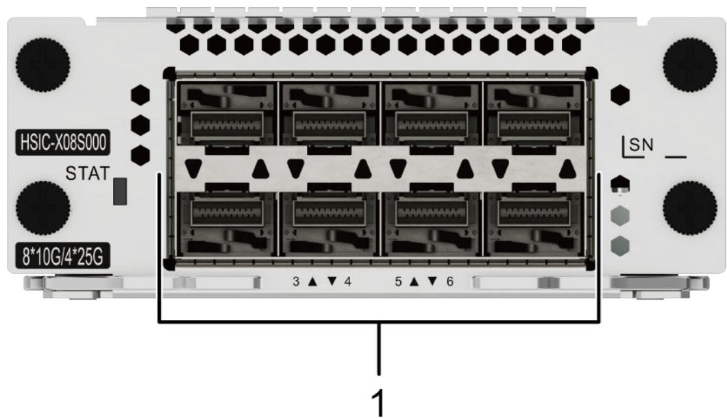
Figure 7-3 Ports on the HSIC-X08S000
