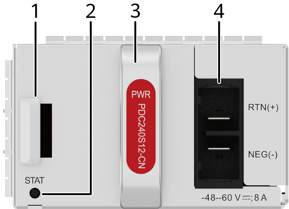
Figure 5-14 Panel of the PDC240S12-CN
