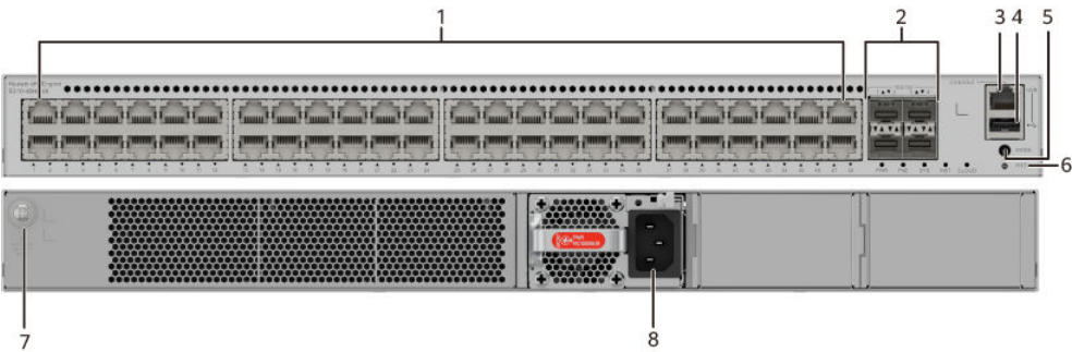
Figure 4-72 S310-48HP4X appearance
