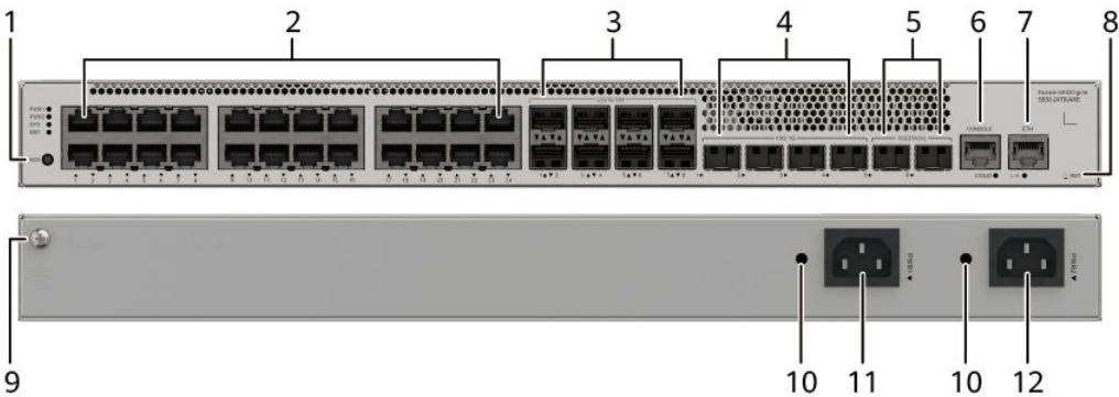
Figure 4-78 S530-24T8J4XE appearance
