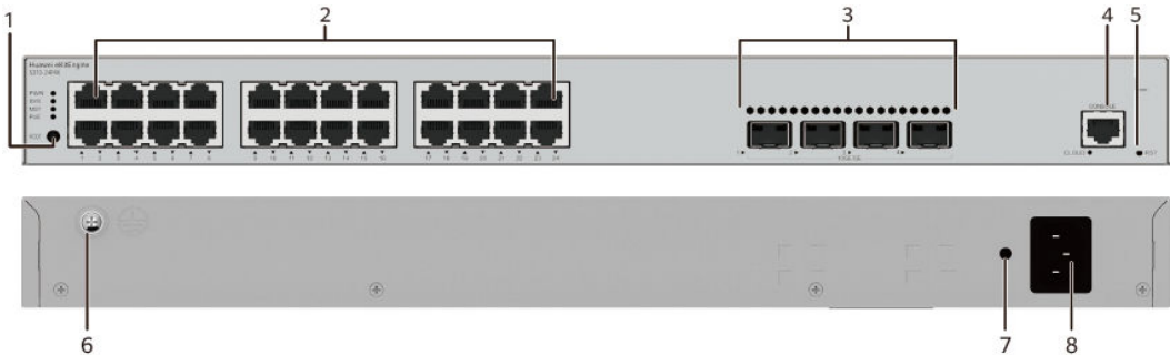
Figure 4-38 S310-24P4X appearance
