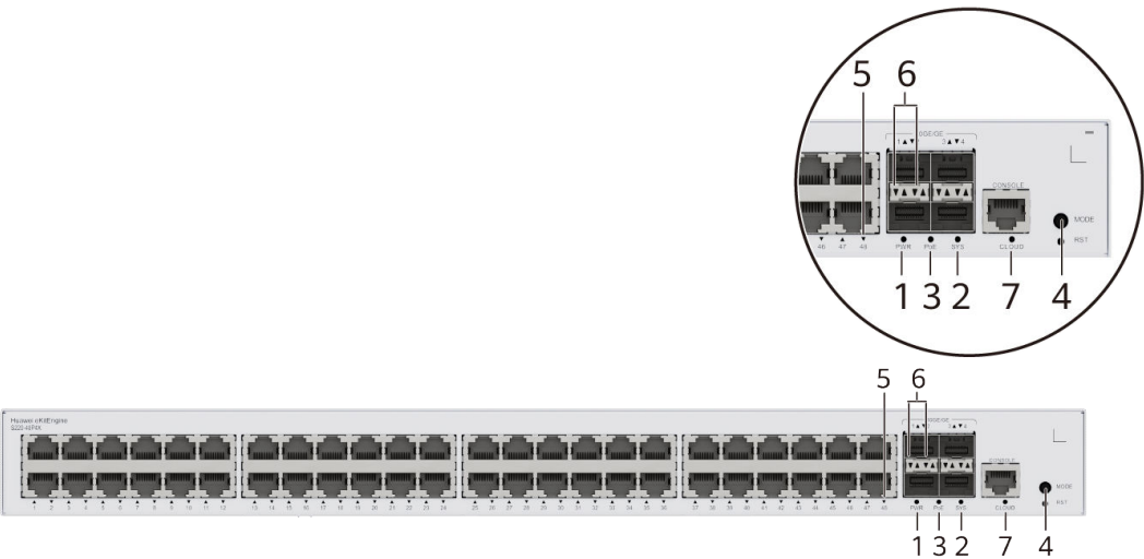
Figure 4-17 Indicators on the Switch
