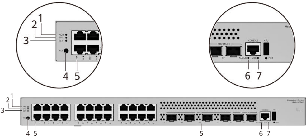
Figure 4-77 Indicators on the Switch
