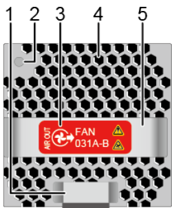
Figure 6-2 Panel of the FAN-031A-B
