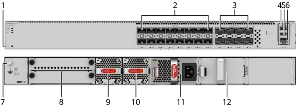
Figure 4-86 S620-16X8YZ appearance
