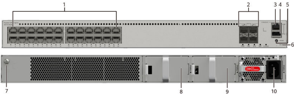
Figure 4-42 S310-24U4X appearance
