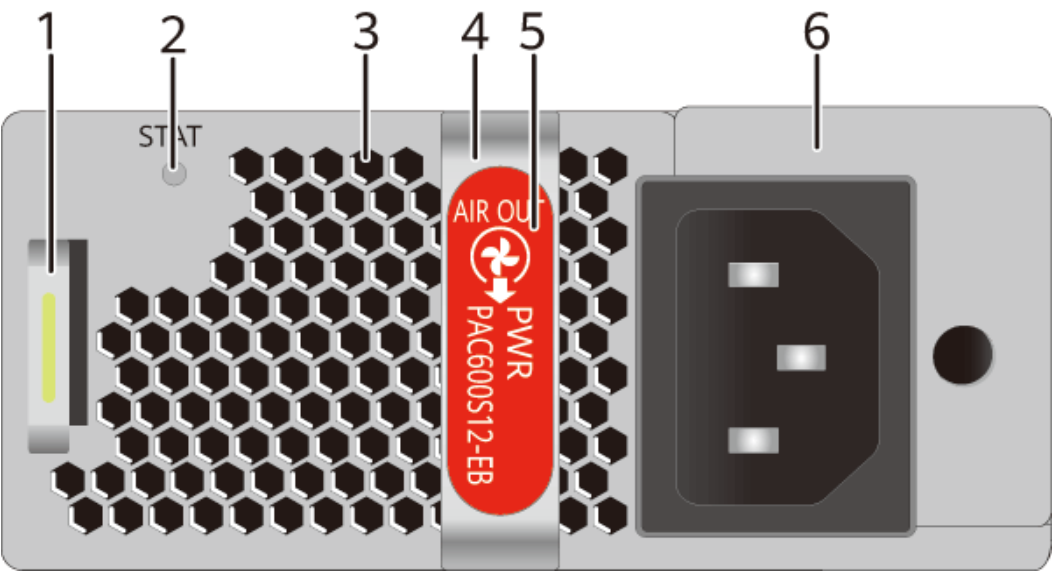
Figure 5-6 Panel of the PAC600S12-EB
