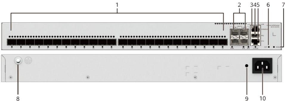
Figure 4-48 S310-24J4X appearance
