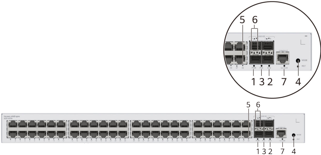
Figure 4-15 Indicators on the Switch
