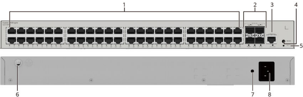
Figure 4-22 S220-48P4X appearance
